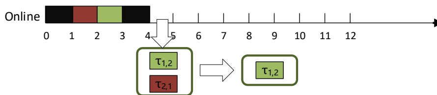
Figure 5.5. The scenario for resizing the waiting queue when some tasks are going to miss their deadlines. The rectangle denotes the waiting queue. Since \tau_{1,2} or \tau_{2,1} will miss its deadline if \tau_{3,1} executes, we do not allow \tau_{3,1} to execute in this scheduling point.
