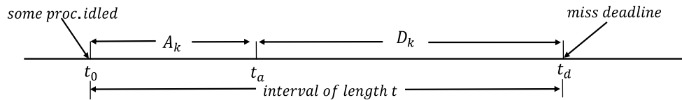
Figure 3.3. A job of task \tau_k with arrival time at t_a and misses its deadline at t_d . t_0 is the time instant that at least one of the m processor is idle.
